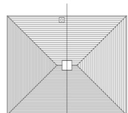
Roof Plan
